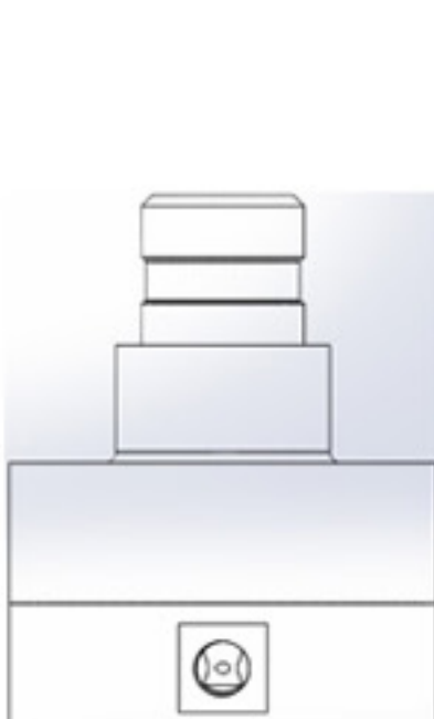
Size 50 – 8" Bore – 3" Hose Plus: 2" Hose & 80 OD Tube options
